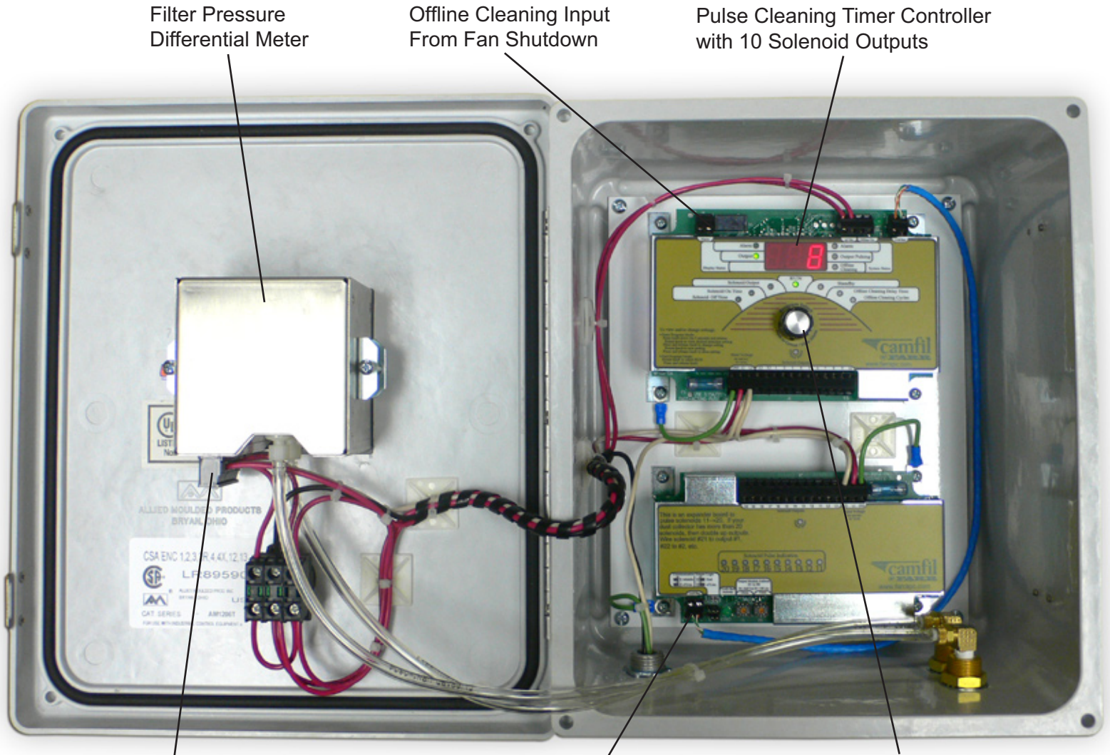
Expander Board for Additional 10 Solenoid Outputs
